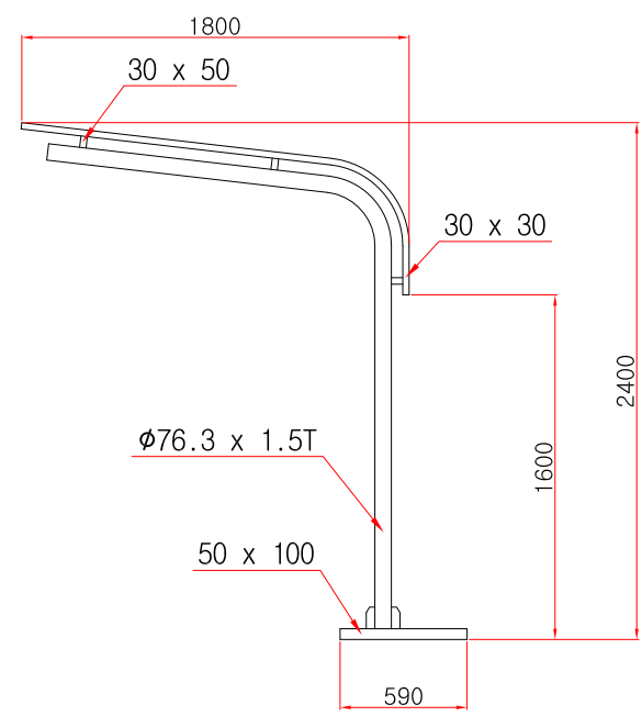
⊕ SIDE ELEVATION SCALE : NONE
